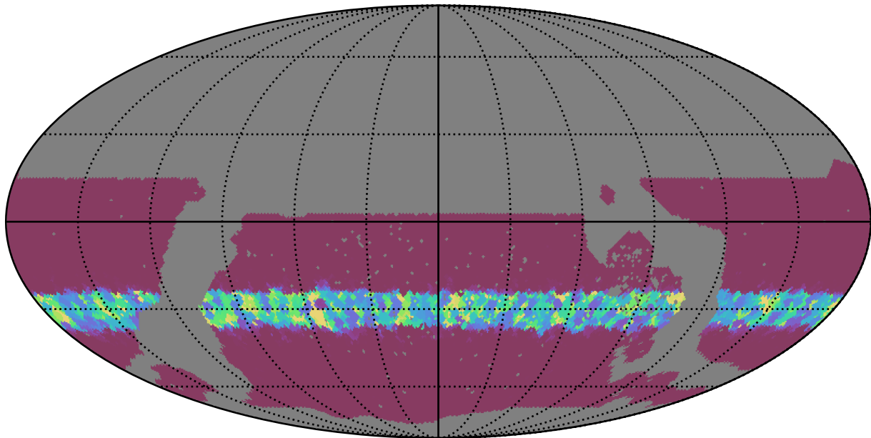
noroll_v3.4_10yrs WFD r band: Min normairmass
