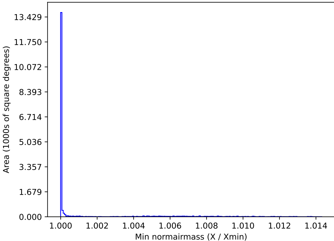
noroll_v3.4_10yrs WFD r band: Min normairmass
