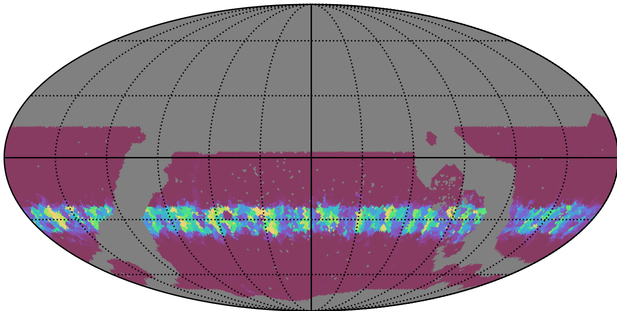
noroll_v3.4_10yrs WFD g band: Min normairmass
