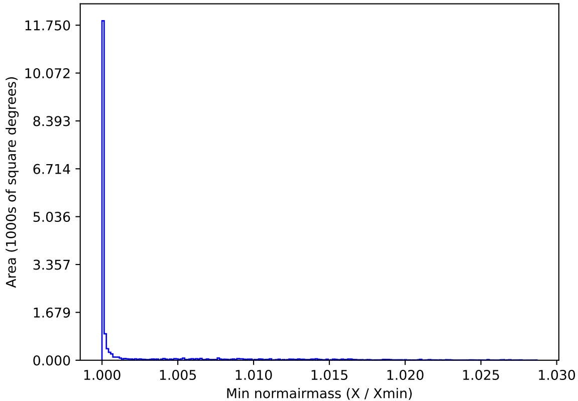
noroll_v3.4_10yrs WFD g band: Min normairmass
