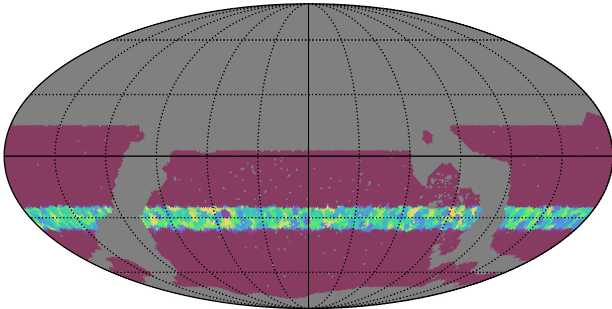
noroll_v3.4_10yrs WFD all bands: Min normairmass
