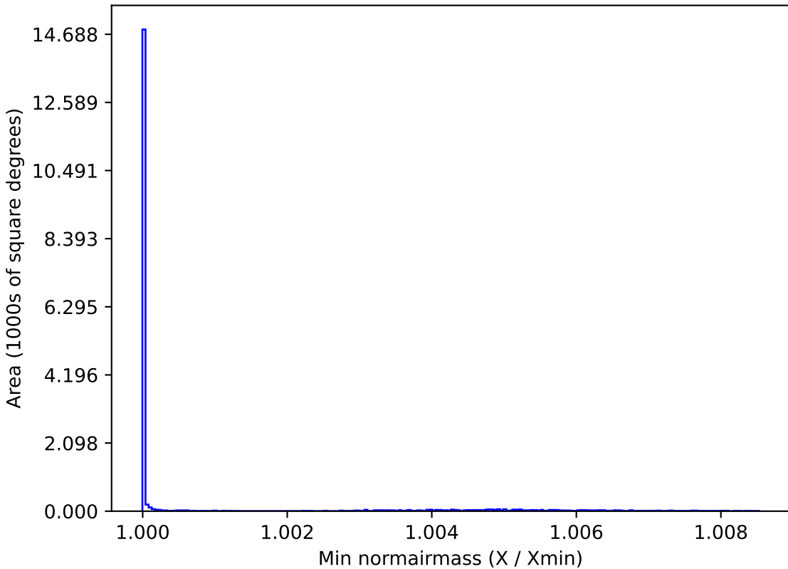
noroll_v3.4_10yrs WFD all bands: Min normairmass
