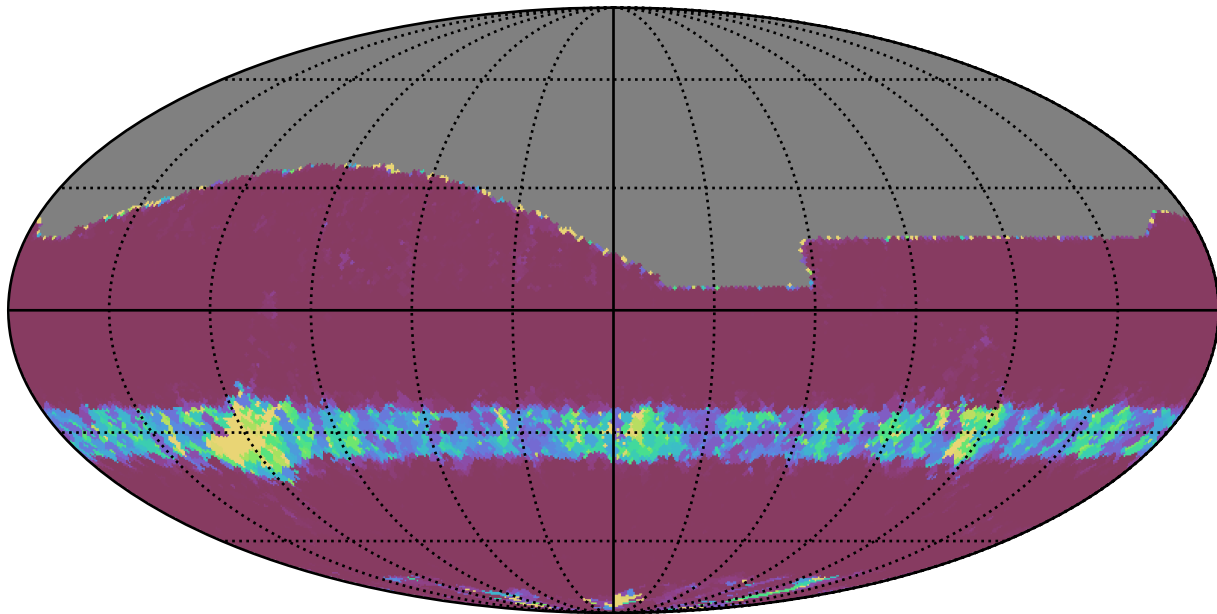
noroll_v3.4_10yrs All sky z band: Min normairmass
