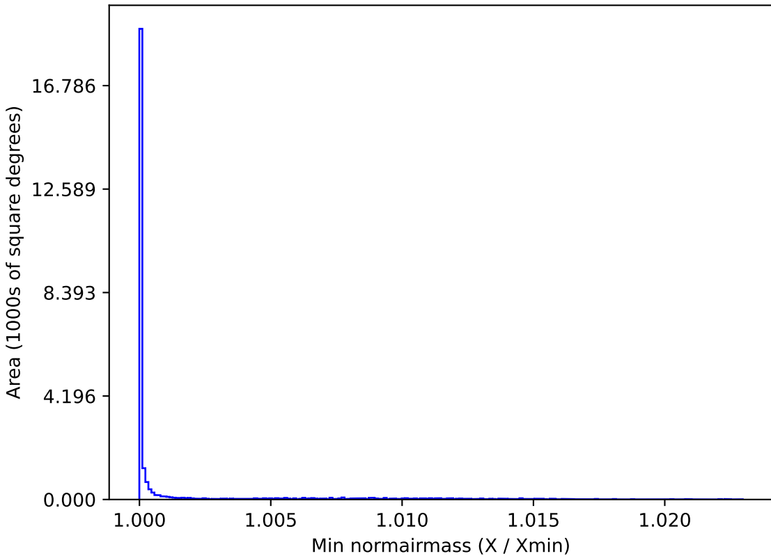
noroll_v3.4_10yrs All sky z band: Min normairmass
