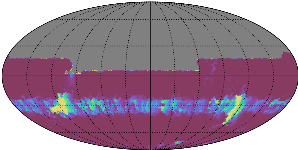
noroll_v3.4_10yrs All sky u band: Min normairmass
