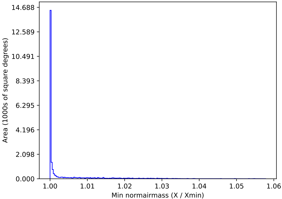
noroll_v3.4_10yrs All sky u band: Min normairmass
