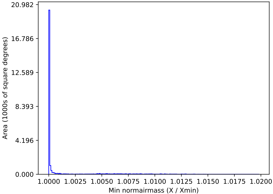
noroll_v3.4_10yrs All sky r band: Min normairmass
