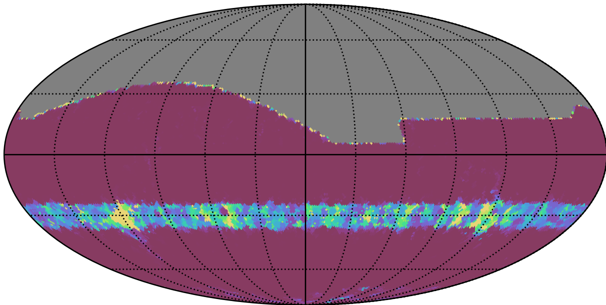
noroll_v3.4_10yrs All sky i band: Min normairmass
