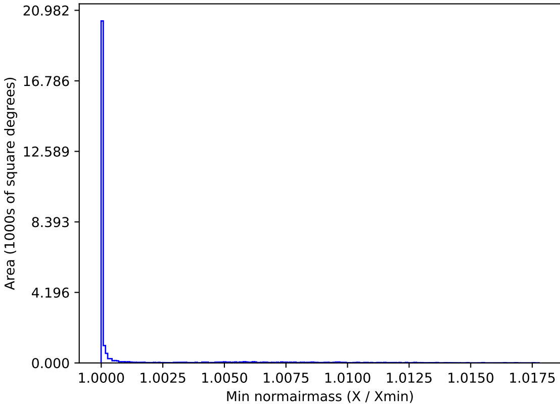
noroll_v3.4_10yrs All sky i band: Min normairmass
