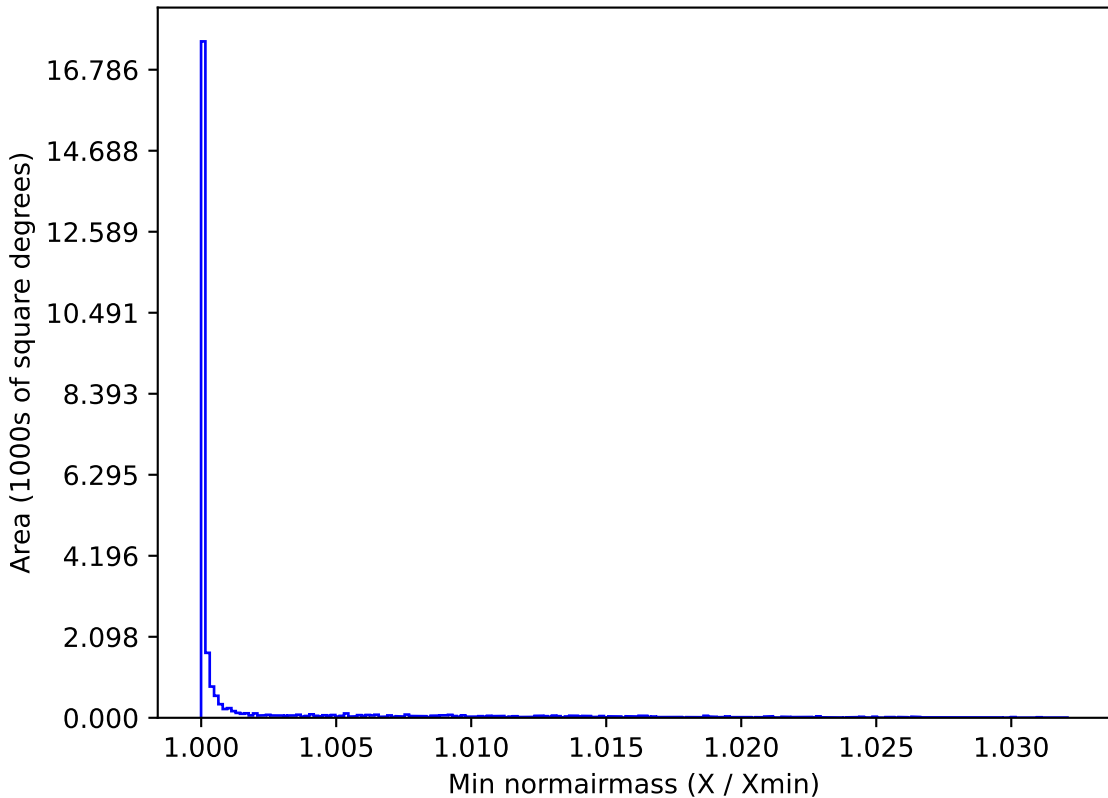
noroll_v3.4_10yrs All sky g band: Min normairmass
