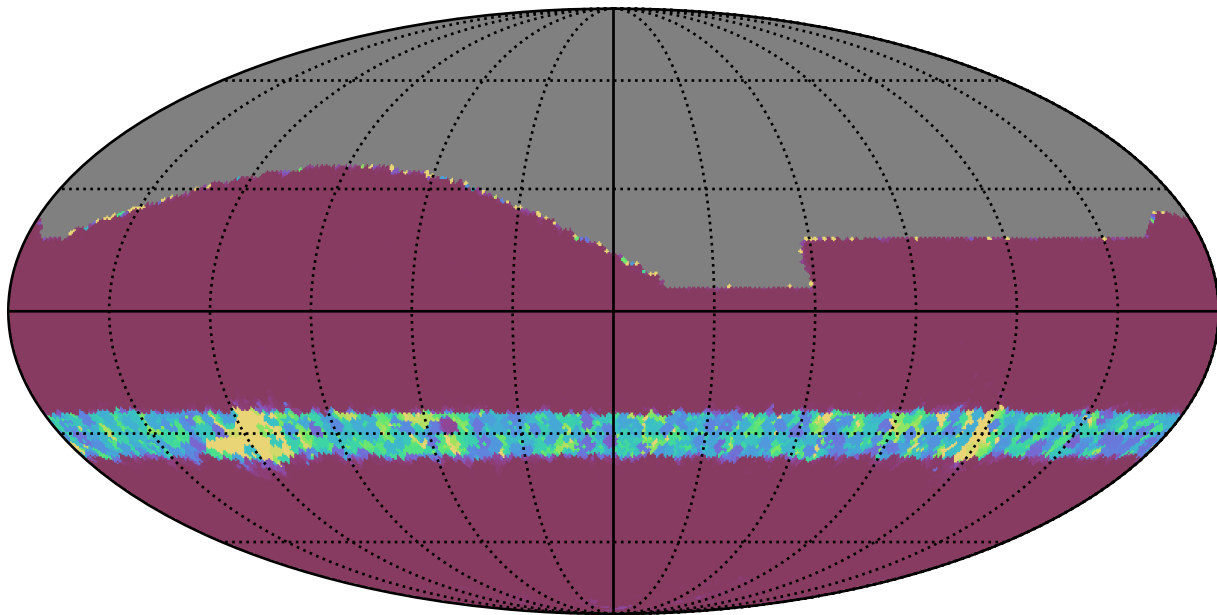
noroll_v3.4_10yrs All sky all bands: Min normairmass
