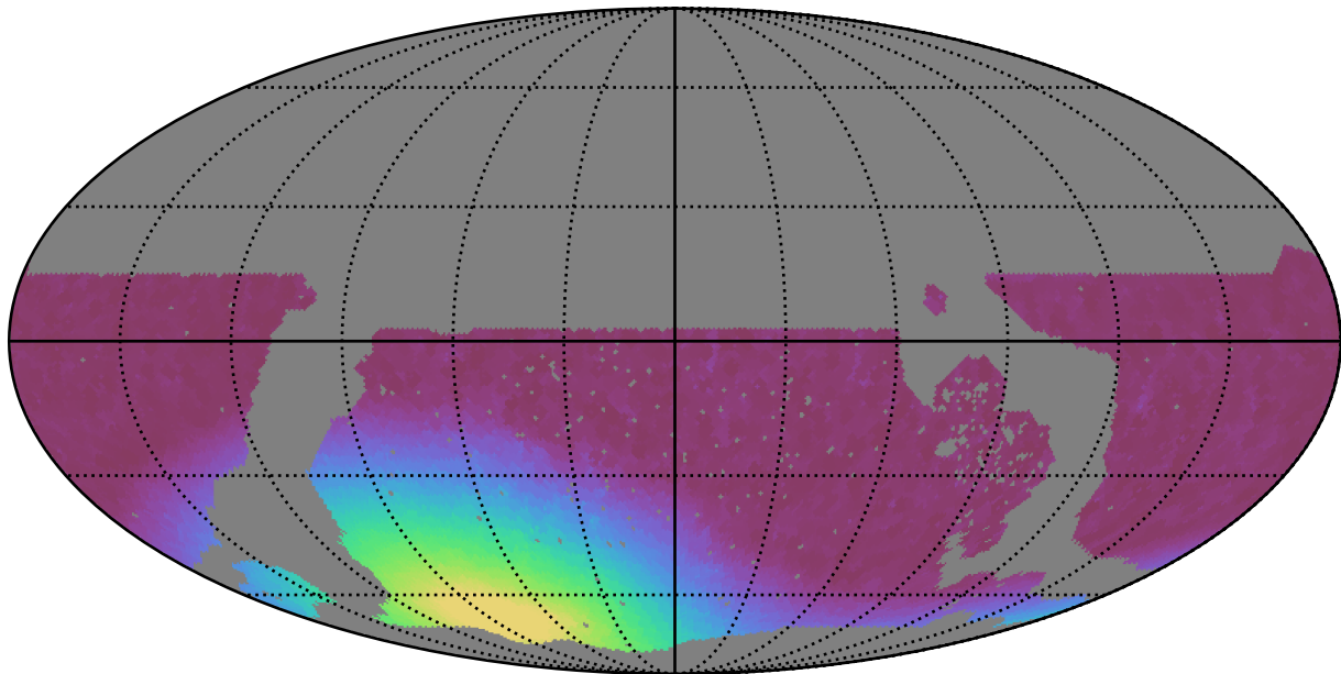
noroll_v3.4_10yrs WFD z band: Min moonDistance
