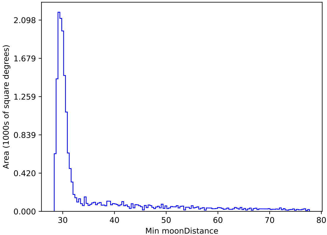
noroll_v3.4_10yrs WFD z band: Min moonDistance
