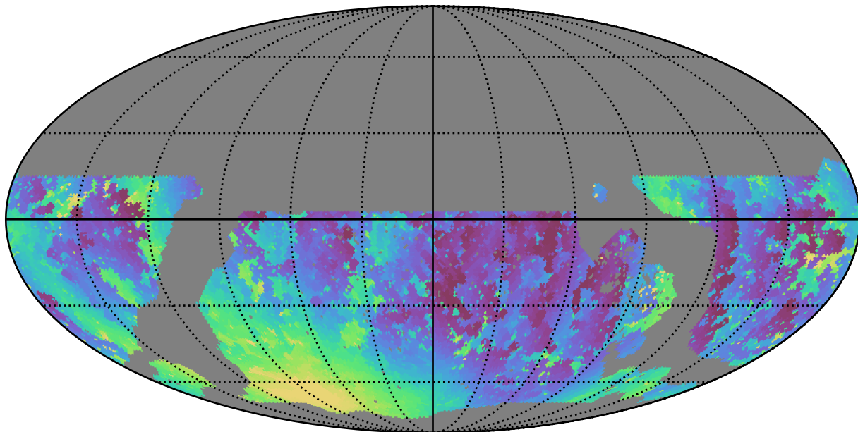
noroll_v3.4_10yrs WFD u band: Min moonDistance
