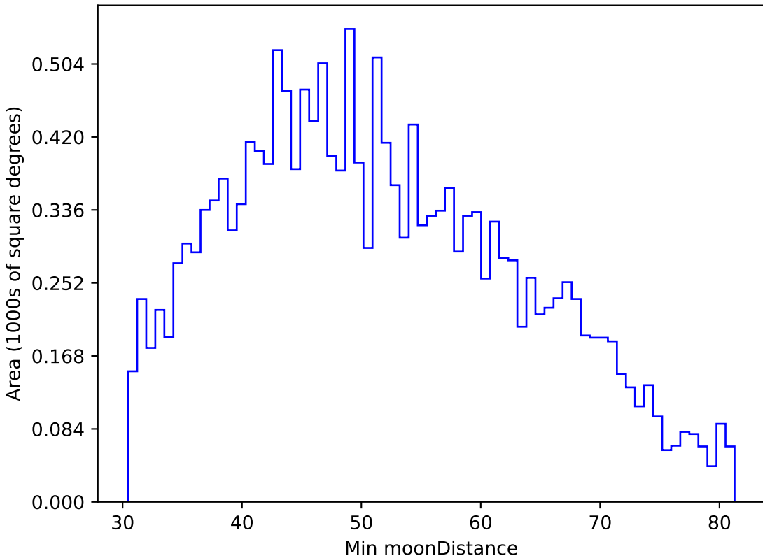
noroll_v3.4_10yrs WFD u band: Min moonDistance
