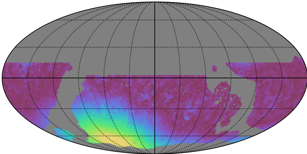
noroll_v3.4_10yrs WFD r band: Min moonDistance
