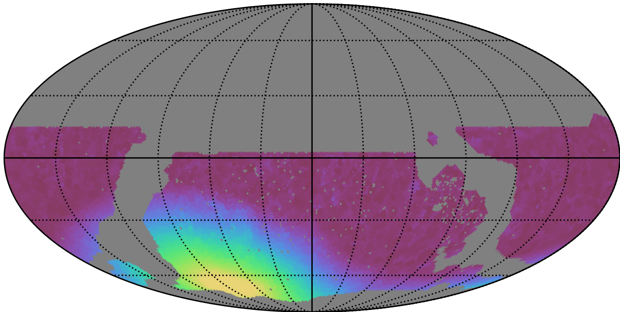
noroll_v3.4_10yrs WFD i band: Min moonDistance
