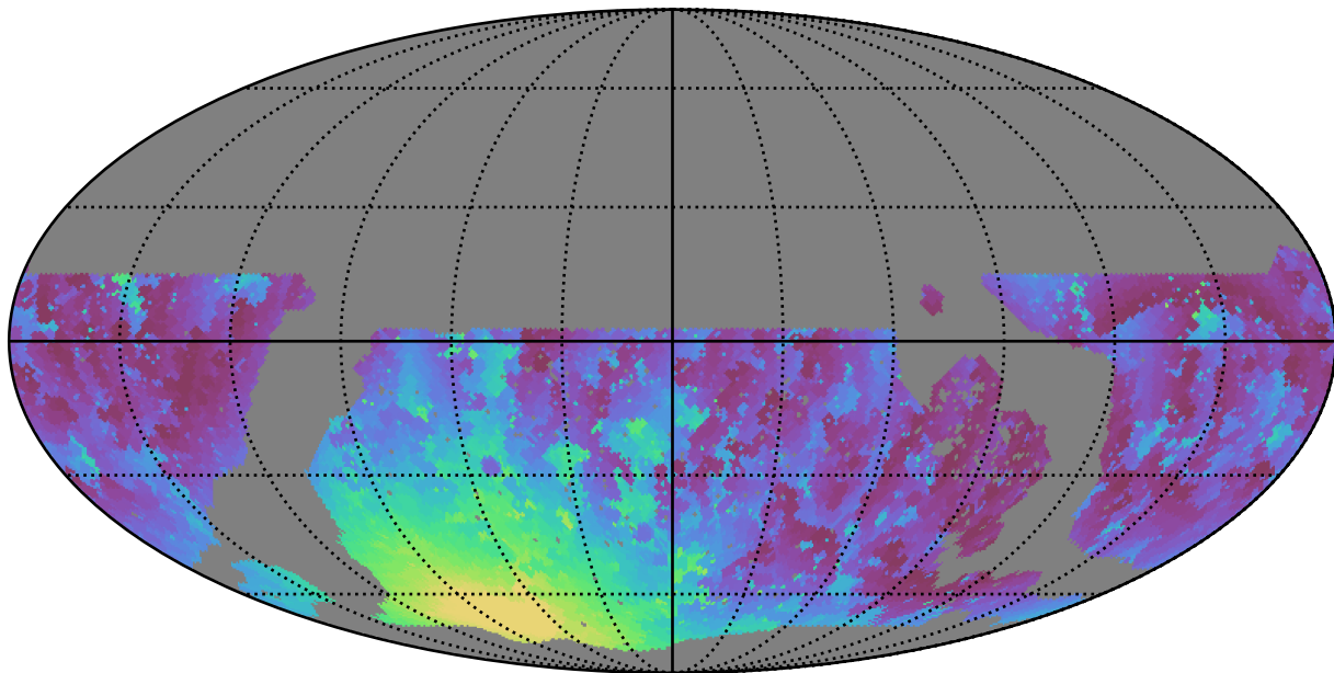
noroll_v3.4_10yrs WFD g band: Min moonDistance
