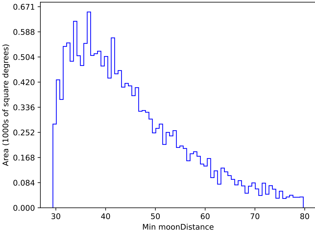
noroll_v3.4_10yrs WFD g band: Min moonDistance
