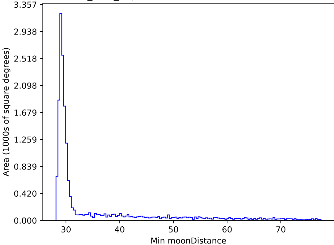
noroll_v3.4_10yrs WFD all bands: Min moonDistance
