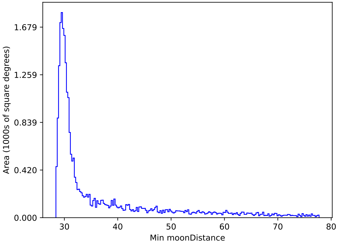
noroll_v3.4_10yrs All sky z band: Min moonDistance
