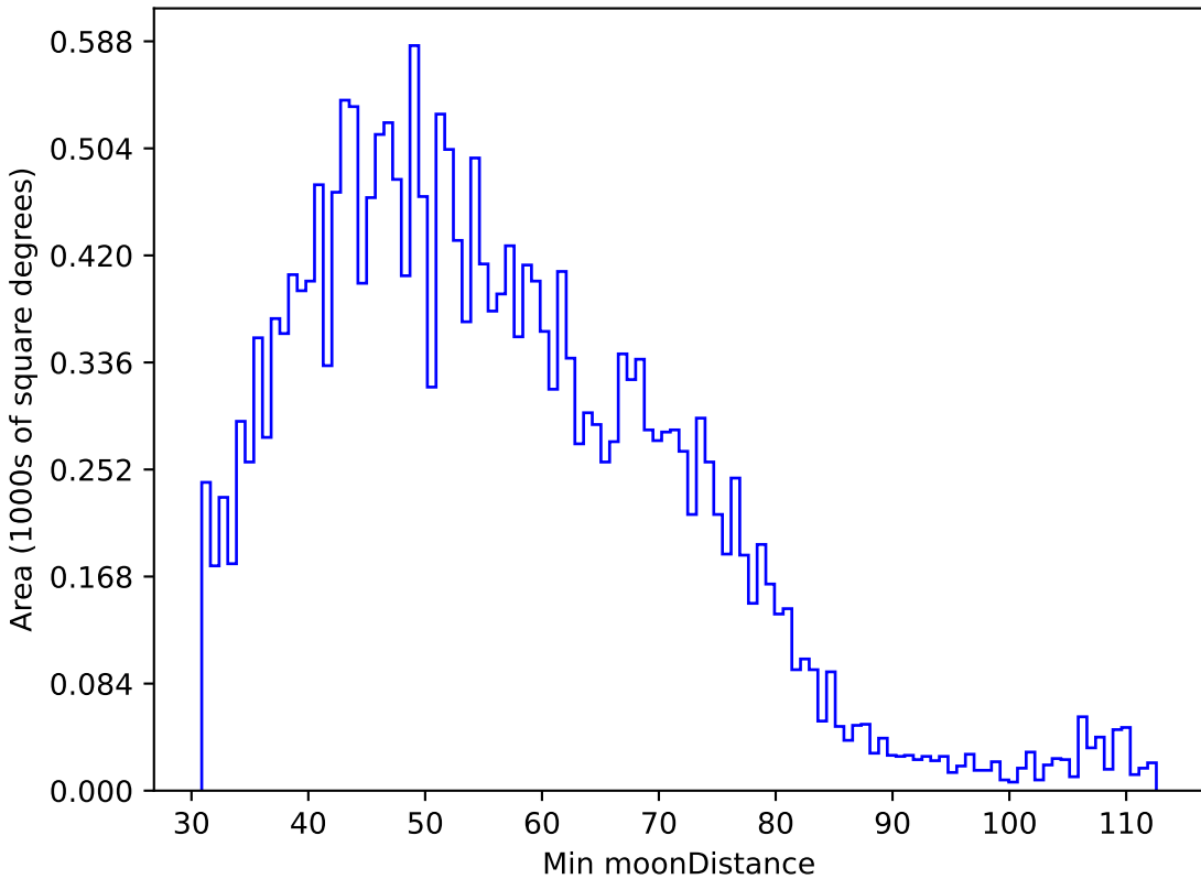
noroll_v3.4_10yrs All sky u band: Min moonDistance
