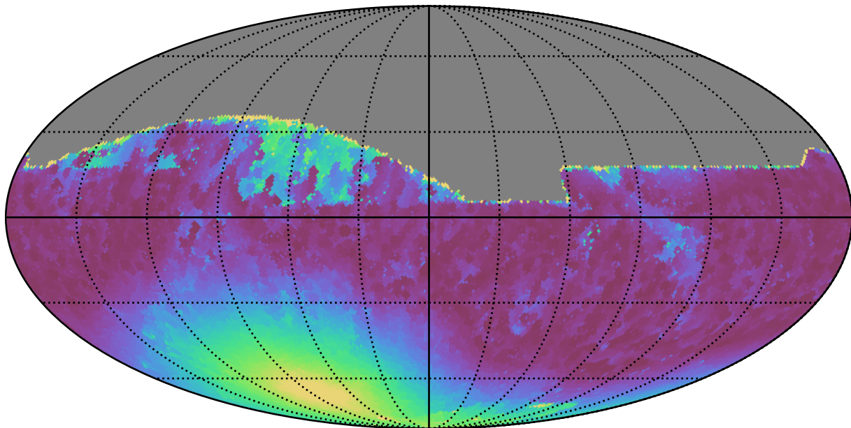
noroll_v3.4_10yrs All sky r band: Min moonDistance
