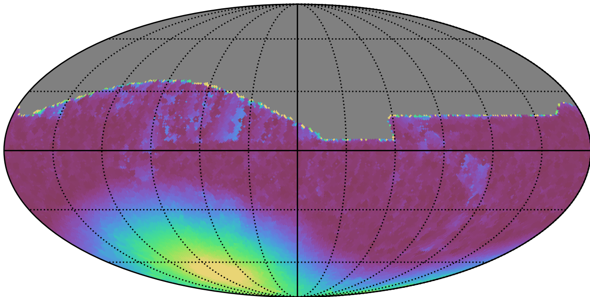
noroll_v3.4_10yrs All sky i band: Min moonDistance
