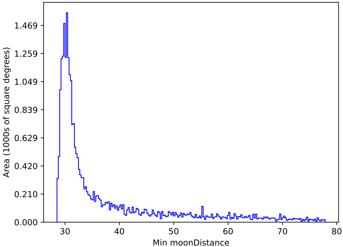
noroll_v3.4_10yrs All sky i band: Min moonDistance
