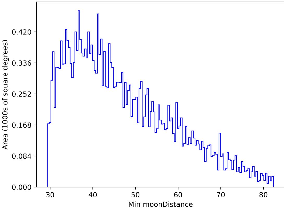
noroll_v3.4_10yrs All sky g band: Min moonDistance
