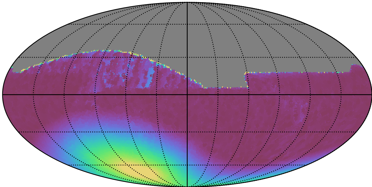
noroll_v3.4_10yrs All sky all bands: Min moonDistance
