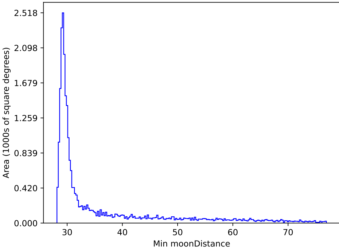
noroll_v3.4_10yrs All sky all bands: Min moonDistance
