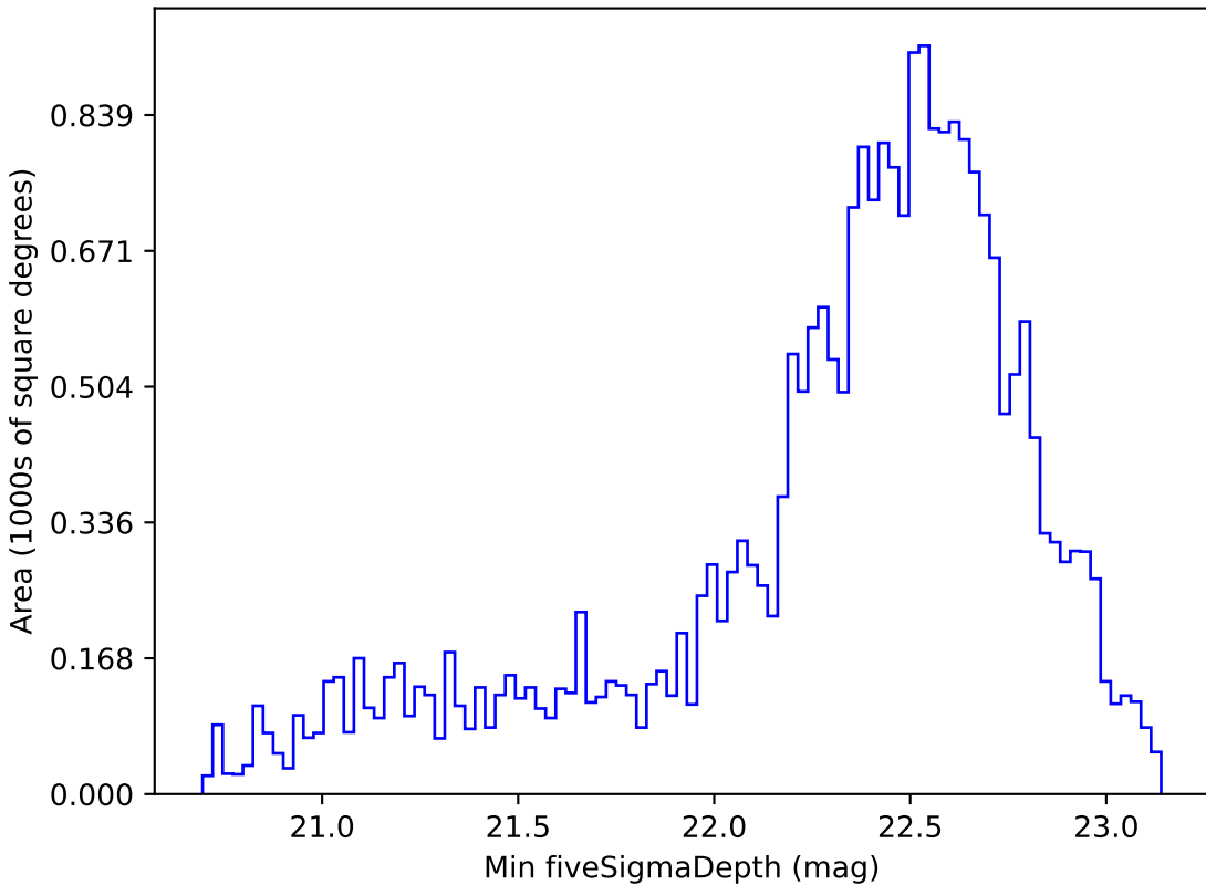
noroll_v3.4_10yrs Yr 1 z band: Min fiveSigmaDepth
