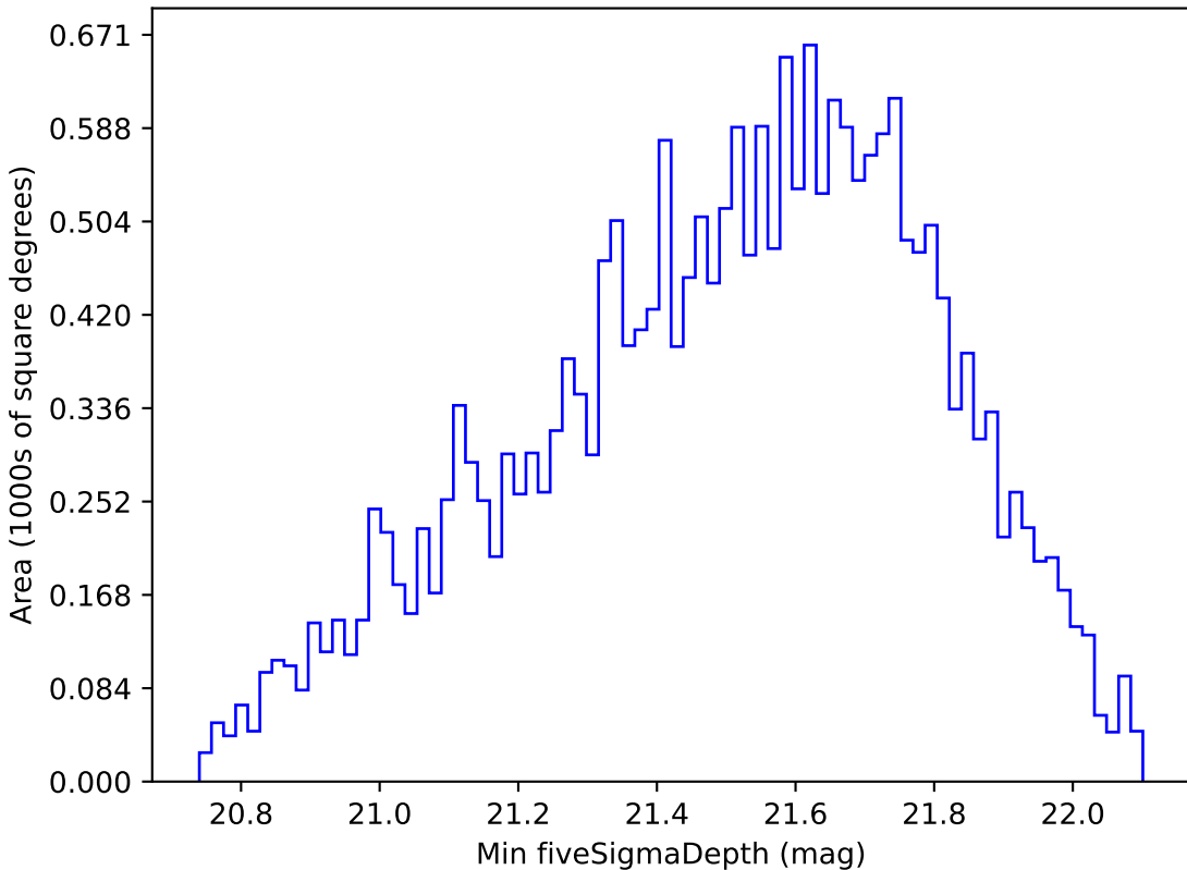
noroll_v3.4_10yrs Yr 1 y band: Min fiveSigmaDepth
