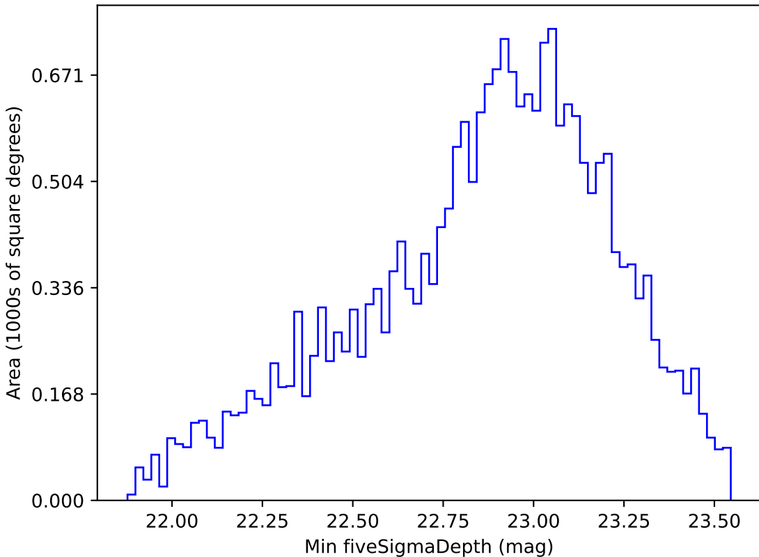
noroll_v3.4_10yrs Yr 1 u band: Min fiveSigmaDepth
