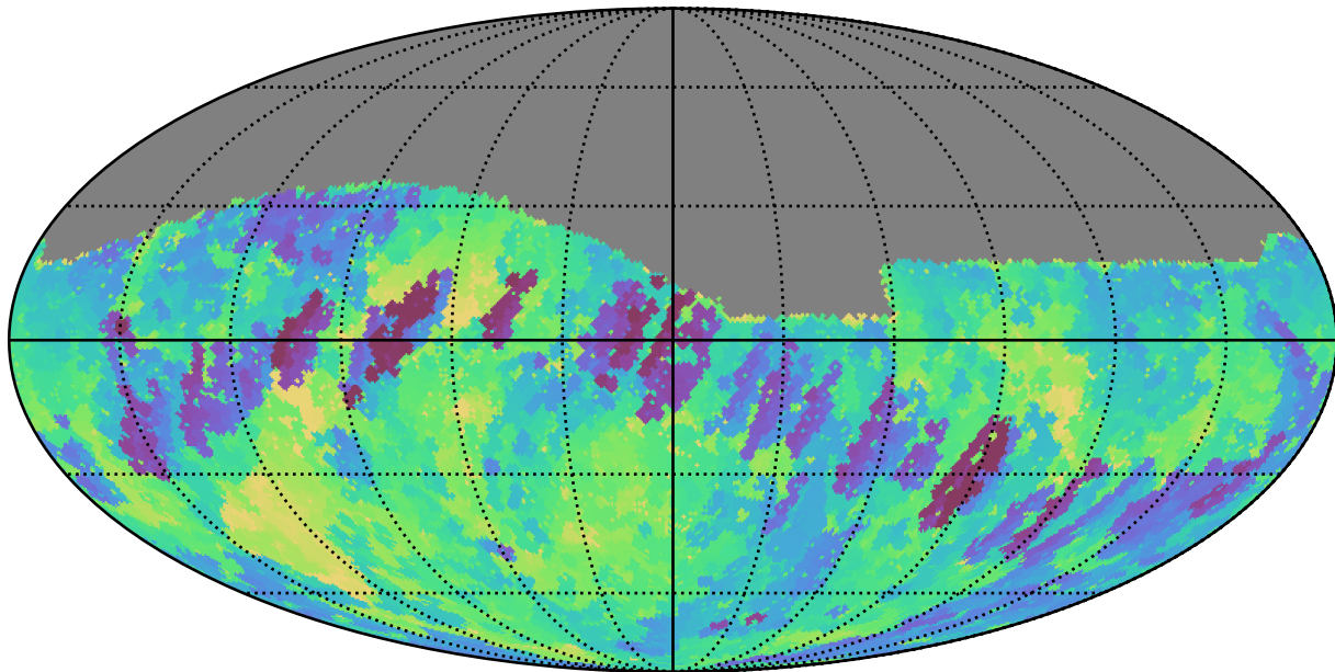
noroll_v3.4_10yrs Yr 1 r band: Min fiveSigmaDepth
