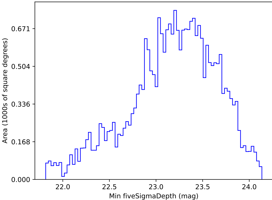
noroll_v3.4_10yrs Yr 1 r band: Min fiveSigmaDepth
