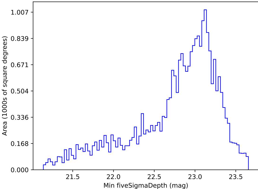
noroll_v3.4_10yrs Yr 1 i band: Min fiveSigmaDepth
