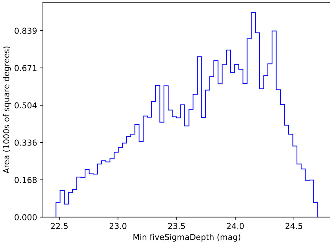
noroll_v3.4_10yrs Yr 1 g band: Min fiveSigmaDepth
