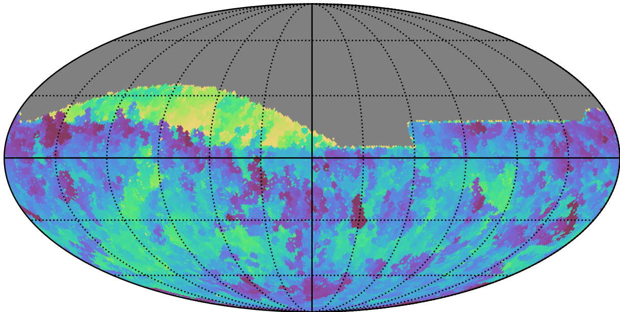
noroll_v3.4_10yrs Yr 1 all bands: Min fiveSigmaDepth
