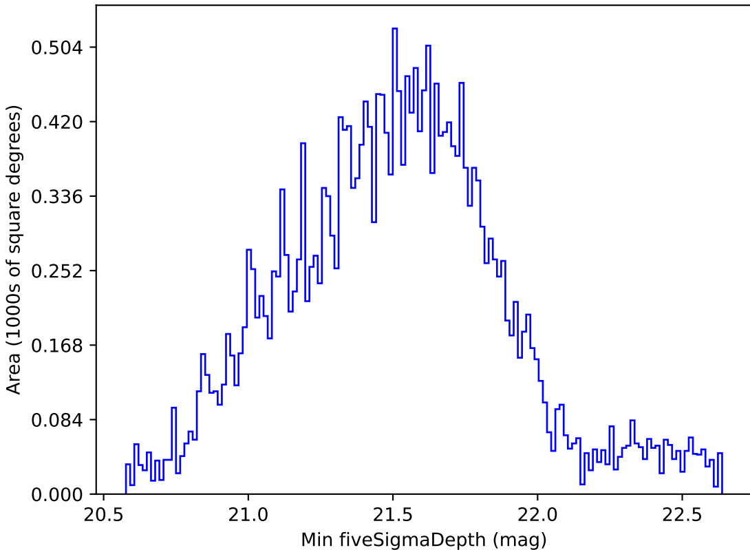
noroll_v3.4_10yrs Yr 1 all bands: Min fiveSigmaDepth
