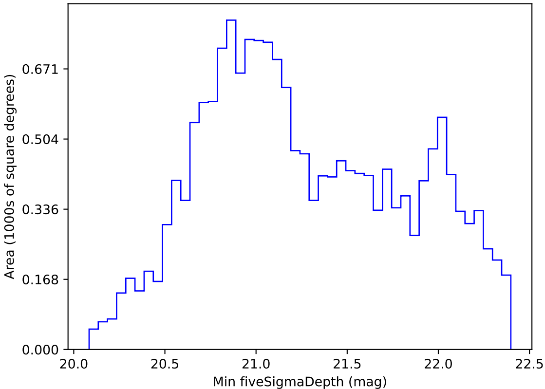
noroll_v3.4_10yrs WFD z band: Min fiveSigmaDepth
