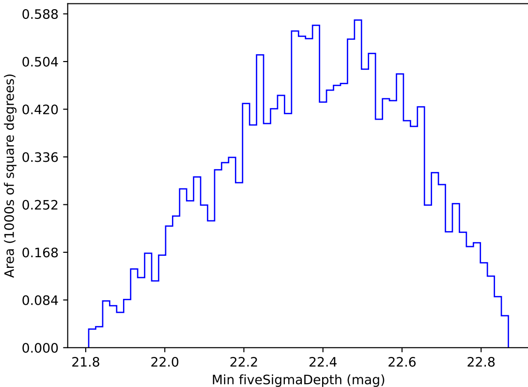
noroll_v3.4_10yrs WFD u band: Min fiveSigmaDepth
