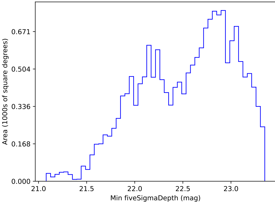
noroll_v3.4_10yrs WFD r band: Min fiveSigmaDepth
