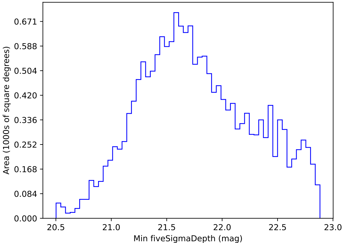
noroll_v3.4_10yrs WFD i band: Min fiveSigmaDepth
