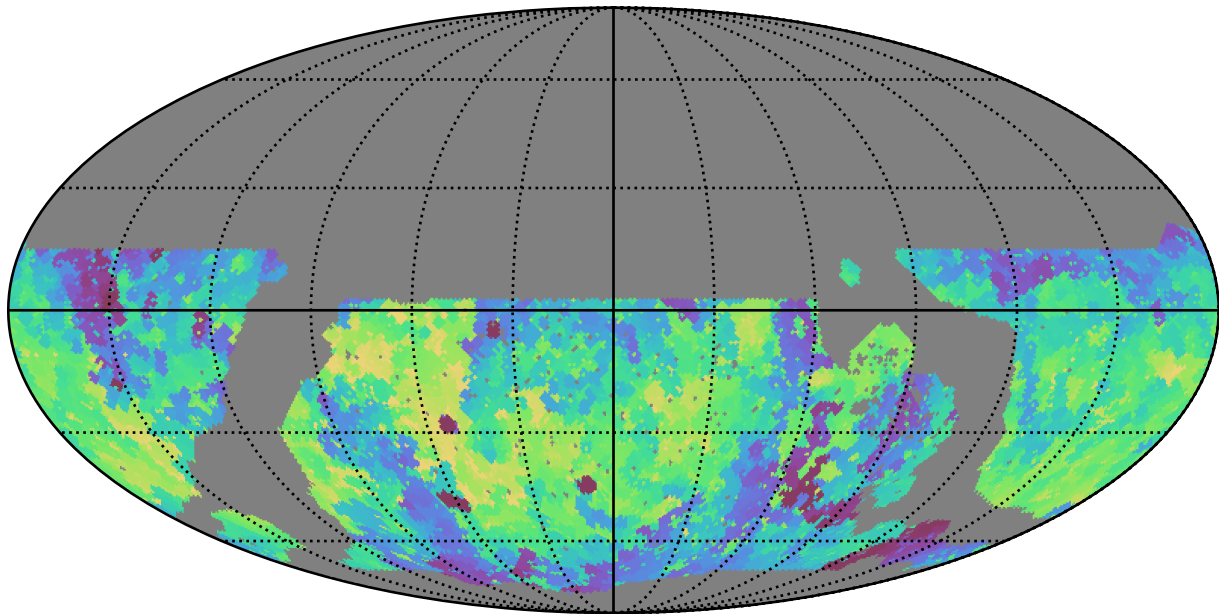
noroll_v3.4_10yrs WFD g band: Min fiveSigmaDepth
