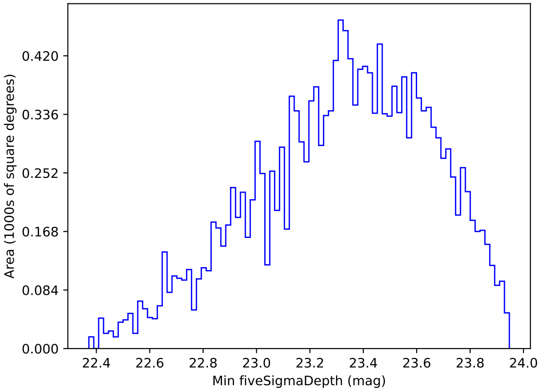
noroll_v3.4_10yrs WFD g band: Min fiveSigmaDepth
