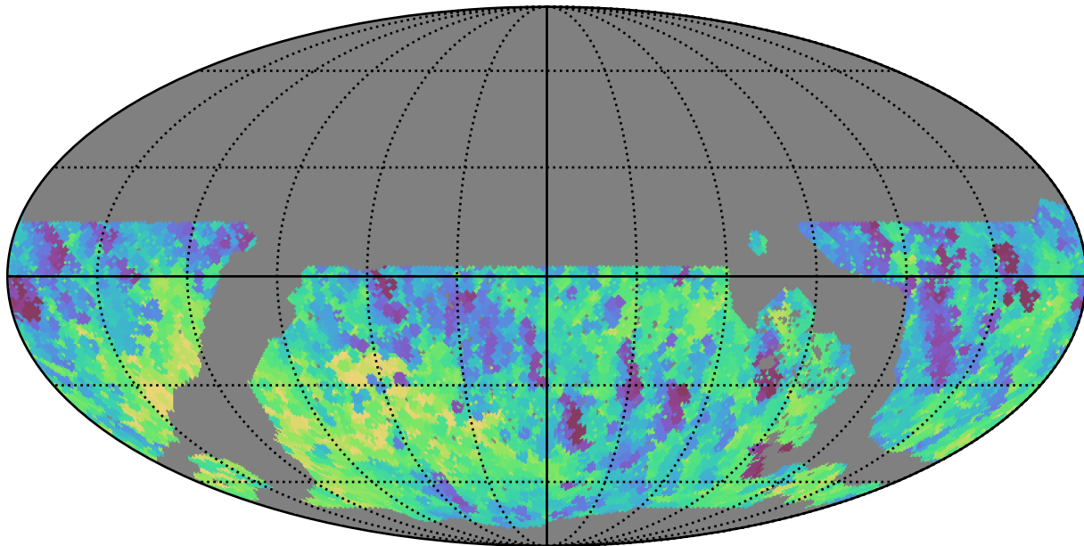
noroll_v3.4_10yrs WFD all bands: Min fiveSigmaDepth
