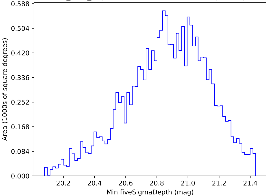
noroll_v3.4_10yrs WFD all bands: Min fiveSigmaDepth
