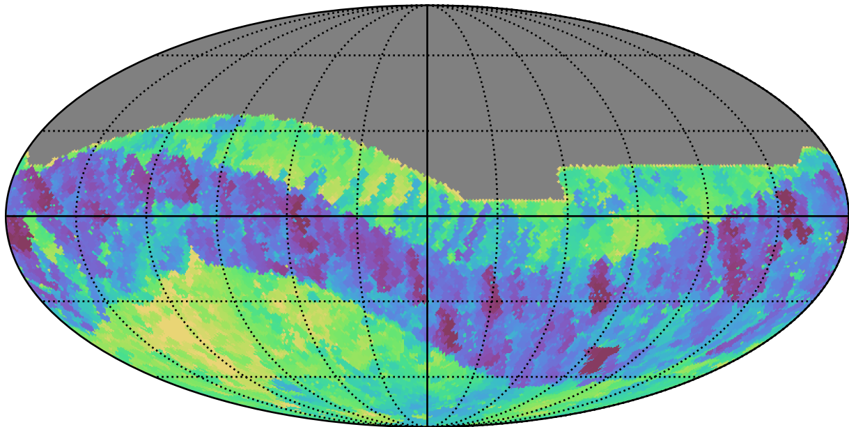
noroll_v3.4_10yrs All sky z band: Min fiveSigmaDepth
